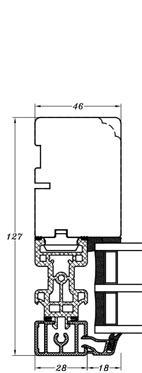
127 mm karm
